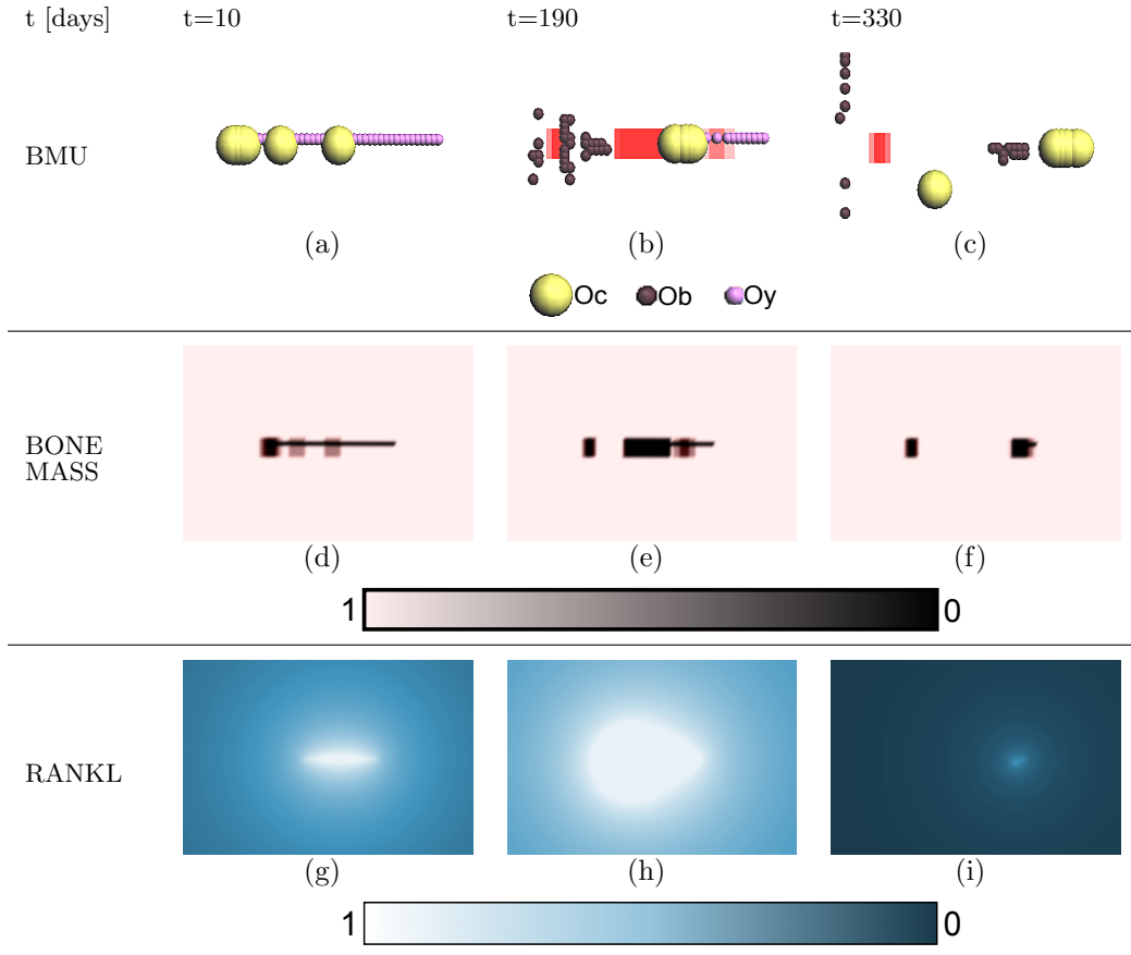
Fig. 2. Model simulation. The first row shows the spatial organization of the BMU; the second row displays the values of bone density; the third row illustrates the RANKL vector field.
